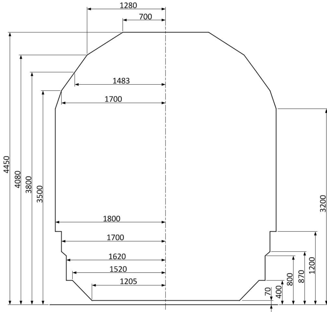
Figure 1: Reference profil of dynamic gauge NO1
