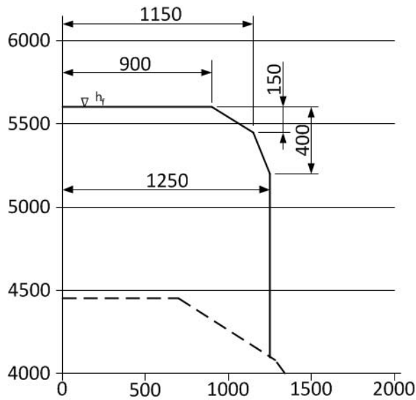
Figure 3: NO1 reference profile for pantograph
